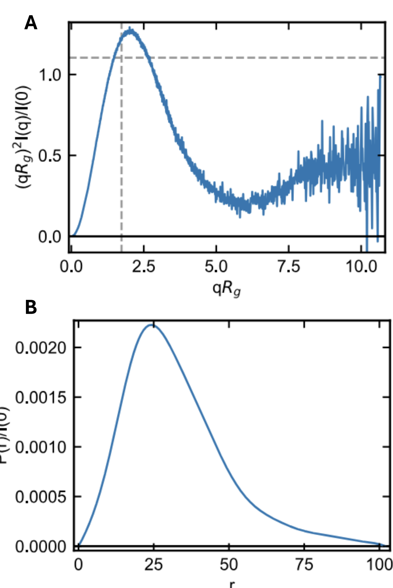
Figure 5: SAXS data summary figure for recombinant human ACTN2 WT ABD. A) Dimensionless Kratky plot. Dashed lines show where a globular system would peak. B) P(r) function(s), normalized by I(0) .
